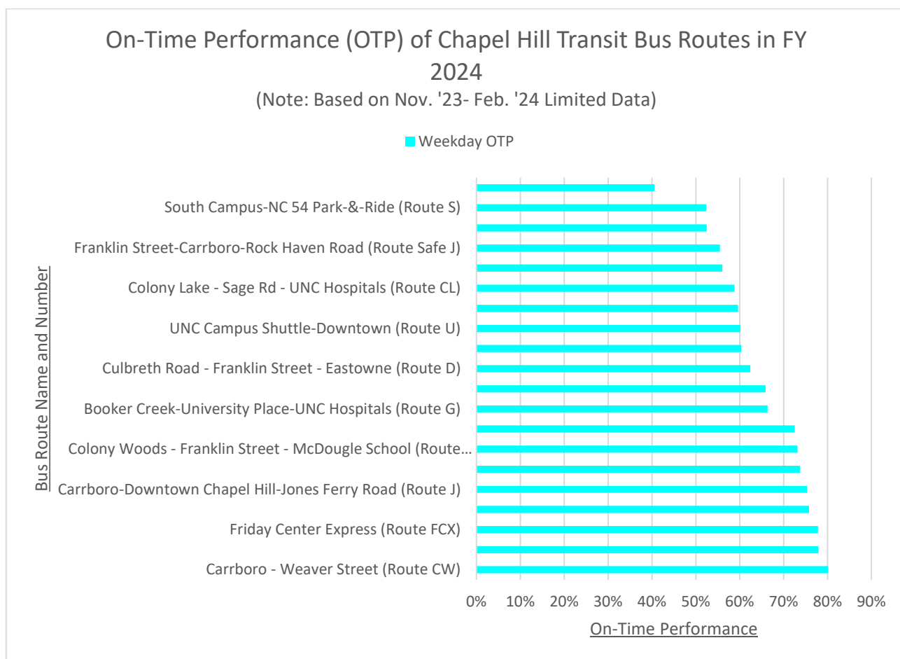
Figure 3.13 Chapel Hill Transit On-Time Performance (FY 2024)
