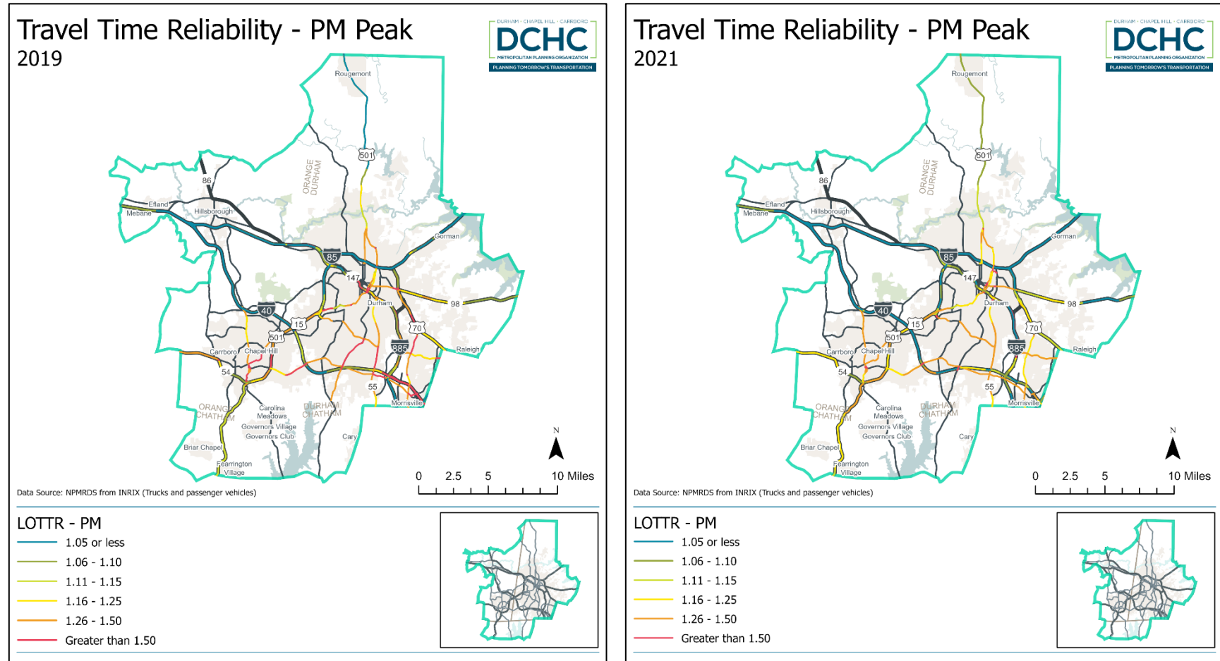
Figure 3.8 Segment LOTTR during PM Peak Period in 2019 and 2021
